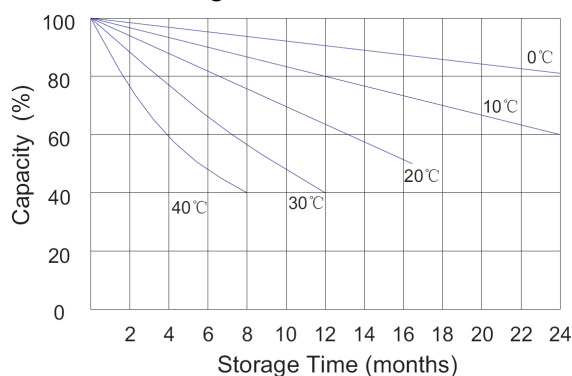
Storage Characteristic Curve
